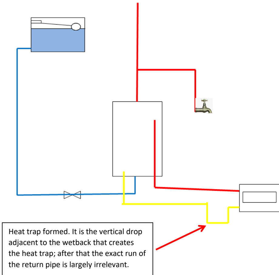
Figure 25. Heat-trap tests.
