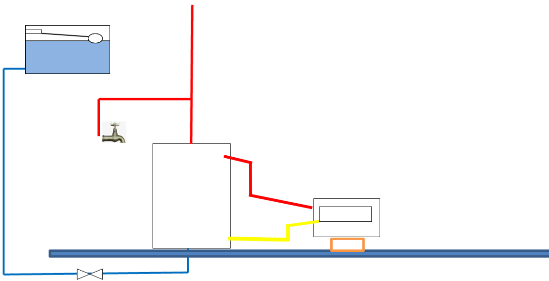
Figure 14. The flow pipe has a rising section that prevents backflow when not in use; the return has a similar heat trap.
