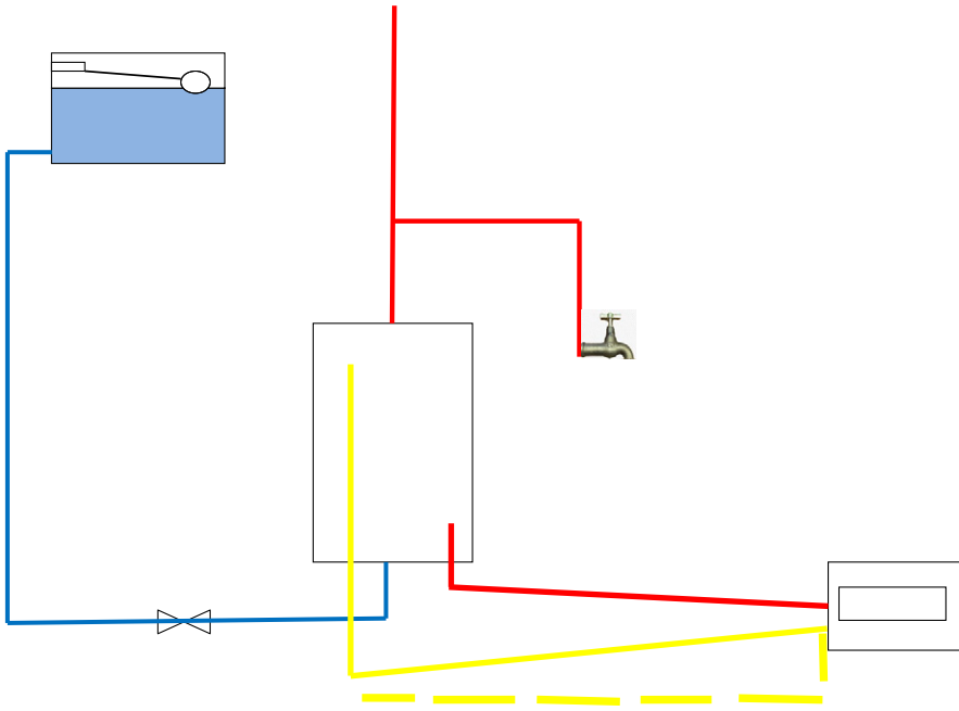
Adjacent direct (rising return). Alternatively, form a heat trap.
